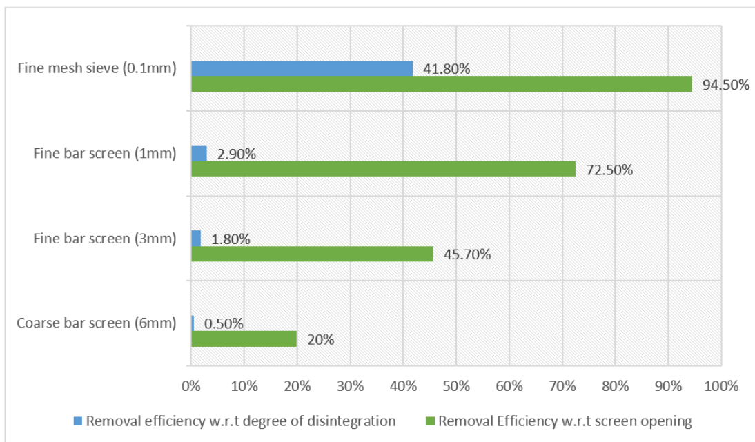
Fig. S3. Removal efficiencies of various filtration screens with respect to screen opening sizes and degree of disintegration.
