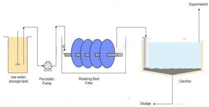
Fig. S4. Schematic of a rotating bed filter.
