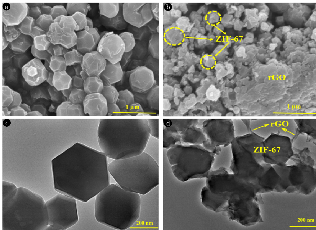
Fig. S1. (a&b) Field-emission SEM micrographs and (c&d) High-resolution TEM images of ZIF-67 and ZIF-67/rGO composite.
