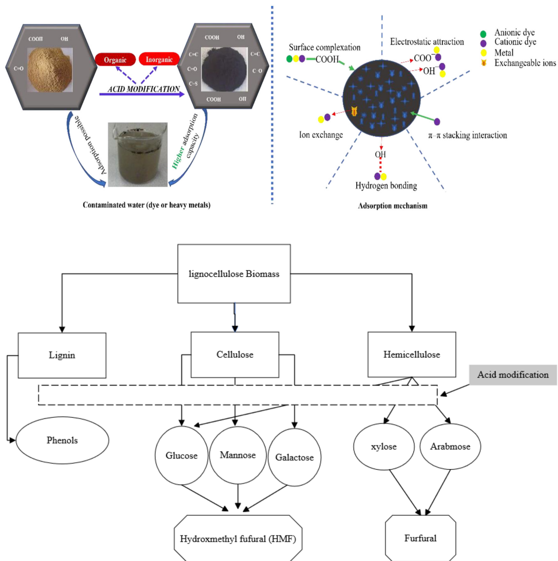
Fig. S1. Schematic description of acid modification mechanism of a LDM.
