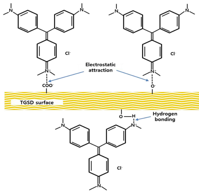
Fig. S2. Proposed interaction of crystal violet dye on Tectona grandis sawdust adsorbent (modified by Ref. [67]).
