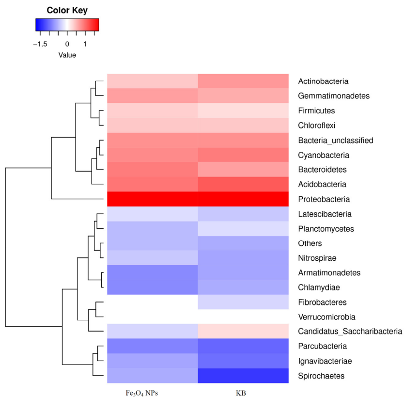
Fig. S1. Heat-map graph of hierarchy cluster for the top 20 phyla in the CWs incorporated with and without Fe 3 O 4 NPs (Fe 3 O 4 NPs represents CWs incorporated with Fe 3 O 4 NPs; KB represents CWs without Fe 3 O 4 NPs). Color intensity in each panel represents the difference and similarity characteristic.
