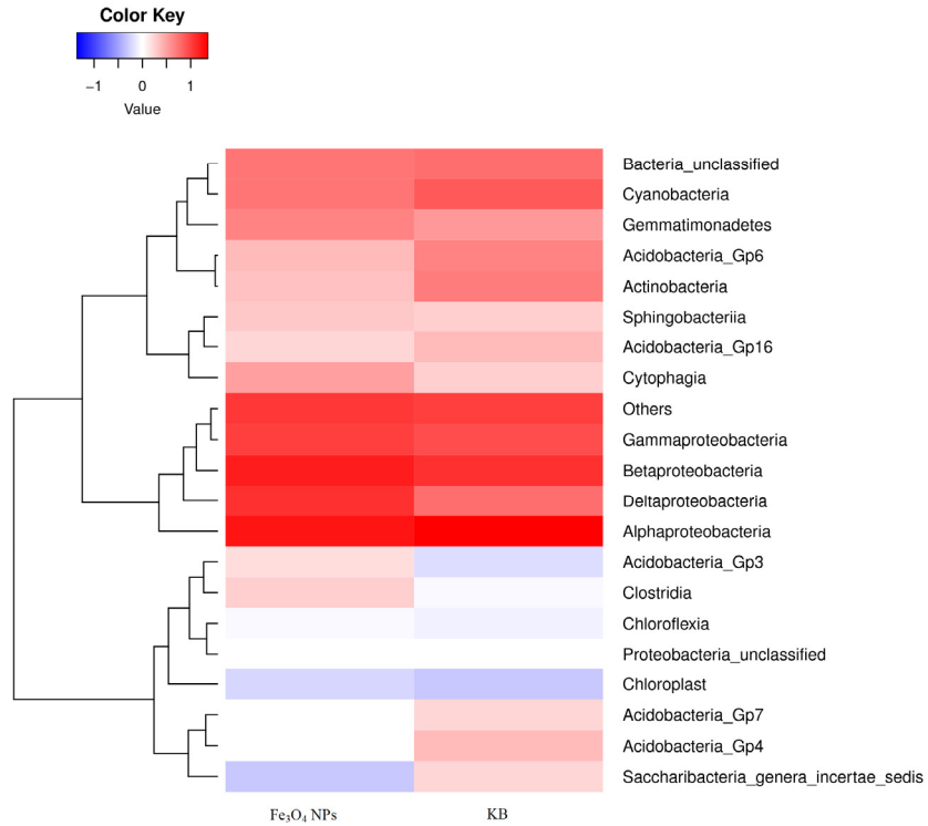
Fig. S2. Heat-map graph of hierarchy cluster for the top 20 classes in the CWs incorporated with and without Fe 3 O 4 NPs (Fe 3 O 4 NPs represents CWs incorporated with Fe 3 O 4 NPs; KB represents CWs without Fe 3 O 4 NPs). Color intensity in each panel represents the difference and similarity characteristic.
