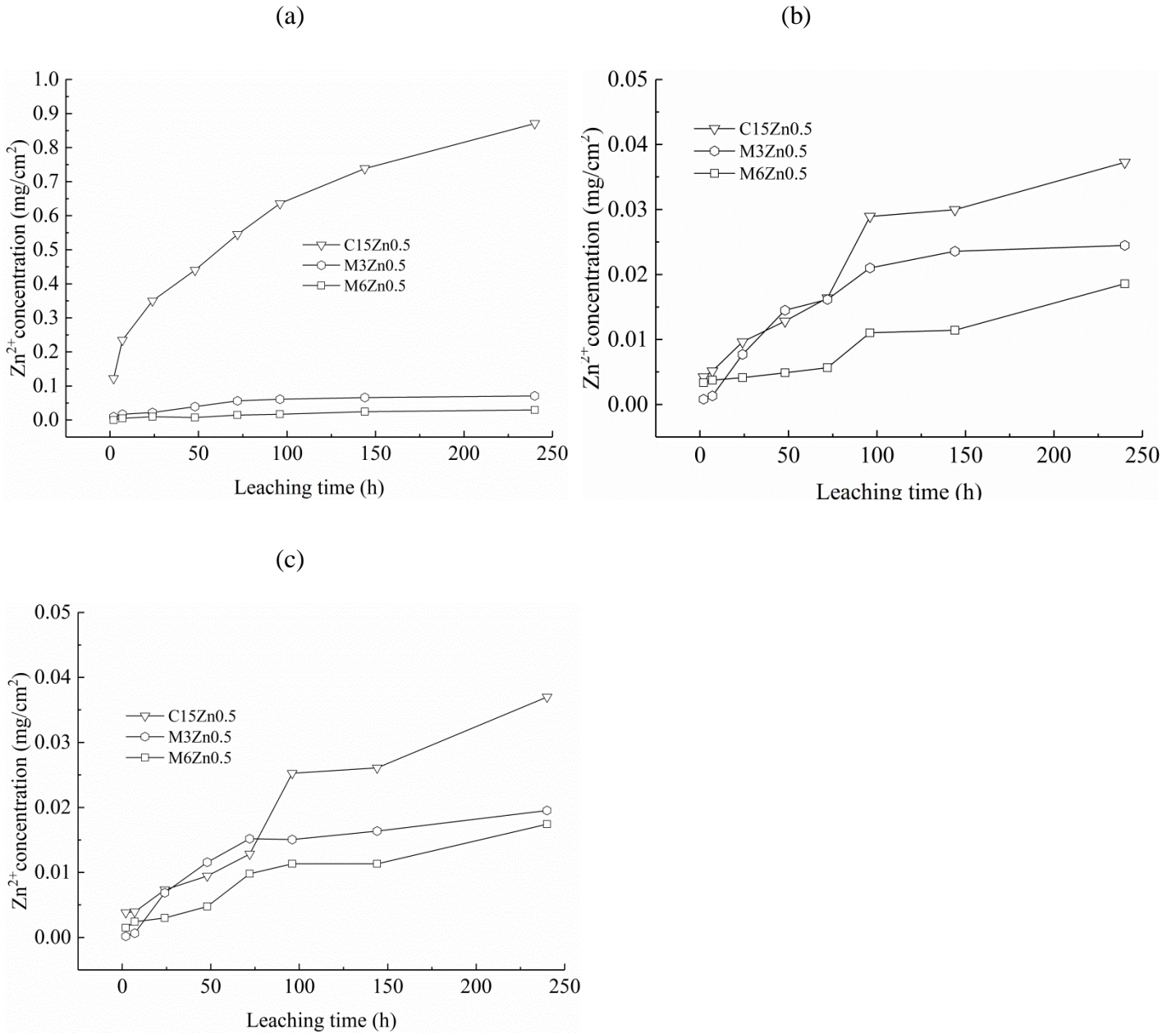
Fig. S2. Total dissolved Zn^{2+} on the surface of the solidified zinc-contaminated soil sample (Ding [31]), (a) Initial pH = 2, (b) Initial pH = 4, (c) Initial pH = 7.
