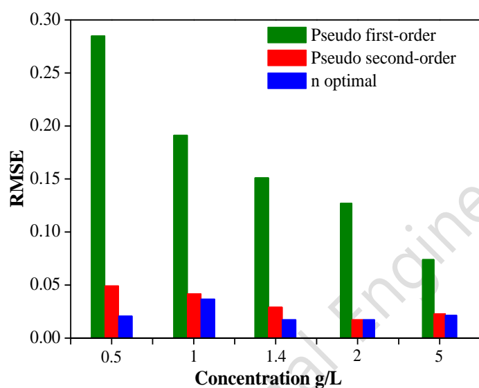
Fig. 4. Comparison of RMSE for pseudo first order equation, pseudo second order equations and the new model for five experiments ( c = 0.5 \text{ g/L}, 1.0 \text{ g/L}, 1.4 \text{ g/L}, 2.0 \text{ g/L} and 5.0 \text{ g/L} ).
