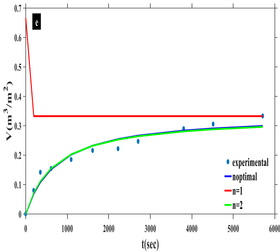
Fig. 3. Adsorption profile of BSA on PCTE membrane plotted for PFO and PSO models during five experiments ((a) c = 0.5\text{g/L} , (b) c = 1.0\text{g/L} , (c) c = 1.4\text{g/L} , (d) c = 2.0\text{g/L} , (e) c = 5.0\text{g/L} ).
