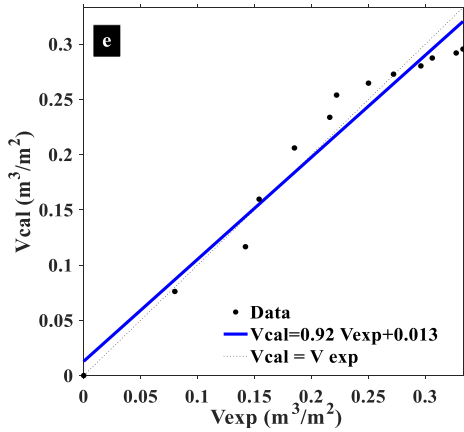
Fig. 2 Nonlinear regression between experimental and calculated volume curves for five experiments (a) c = 0.5\text{ g/L} , (b) c = 1.0\text{ g/L} , (c) c = 1.4\text{ g/L} , (d) c = 2.0\text{ g/L} and (e) c = 5.0\text{ g/L} .
