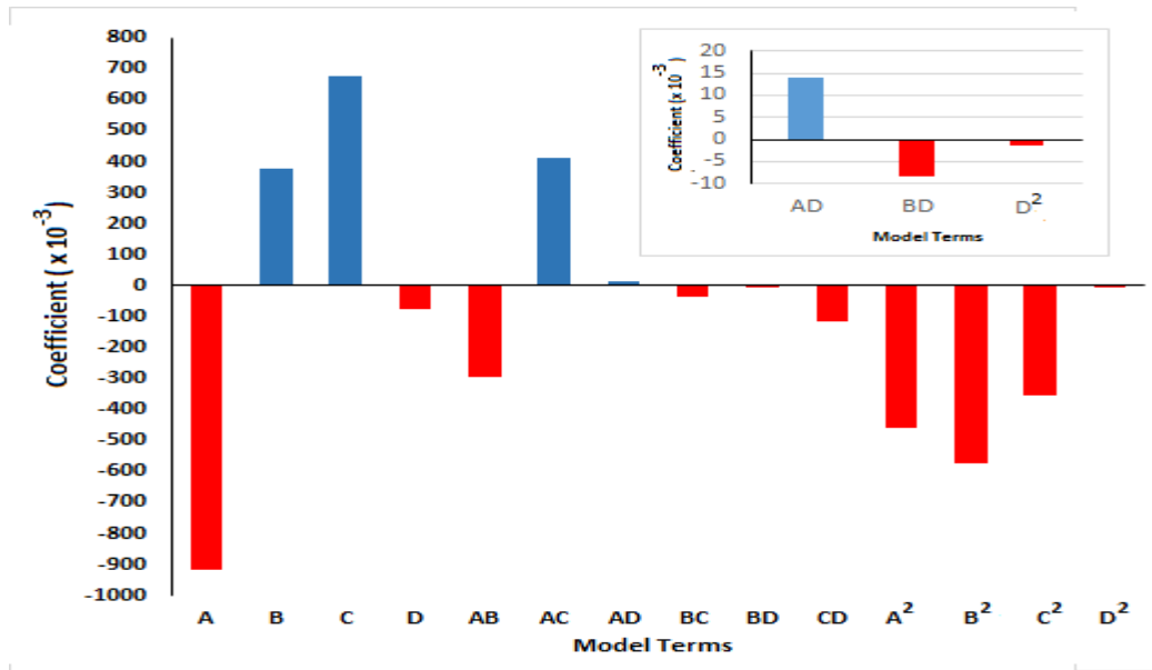
Fig. S1. Impact Pareto plot of model terms.
