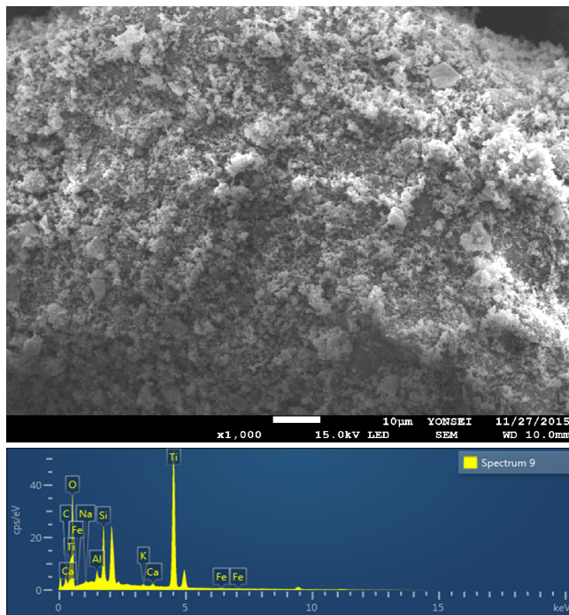
Fig. 2. Scanning electron microscope (SEM) and the energy dispersive X-ray spectrometer images for the TiO 2 coated zeolite.
